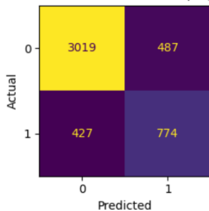
Confusion Matrix — Gini (80/20)
