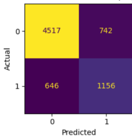
Confusion Matrix — Gini (70/30)
